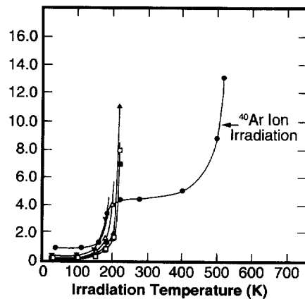
Fig. 3. Dose-to-amorphization in displacements per atom at various irradiation temperatures for 0.9 MeV electron and 0.5–1.5 MeV ^{40}Ar ion ( \bullet ) irradiations of Zr_3Fe . Electron dose rate: \blacksquare , 1.83 \times 10^{-3} dpa s^{-1} ; \square , 1.68 \times 10^{-3} dpa s^{-1} ; \blacktriangle , 1.47 \times 10^{-3} dpa s^{-1} ; \triangle , 1.23 \times 10^{-3} dpa s^{-1} ; \blacktriangledown , 1.04 \times 10^{-3} dpa s^{-1} .
