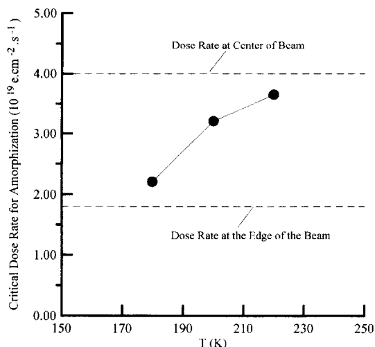
Fig. 8. Critical dose rate for amorphization of Zr_3Fe under electron irradiation as a function of temperature. Also shown is the dose rate variation afforded within the electron beam. [94]
