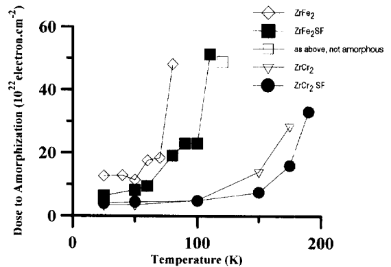
Fig. 10. Dose-to-amorphization versus temperature for ZrCr_2 and ZrFe_2 under electron irradiation, showing the effect of a high density of stacking faults (filled spots) on the amorphization process.
