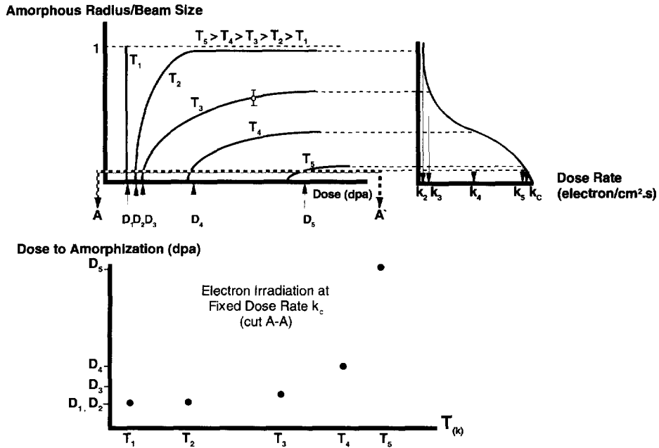
Fig. 5. Schematic plot of amorphous beam radius as a function of dose for several temperatures, showing influence of dose rate and relationship to dose-to-amorphization versus temperature curve.
