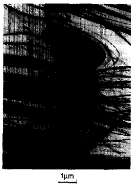
Fig. 11. Triple joint between three Zr_3Fe grains showing preferential amorphization during electron irradiation at 250 keV at 25 K.
