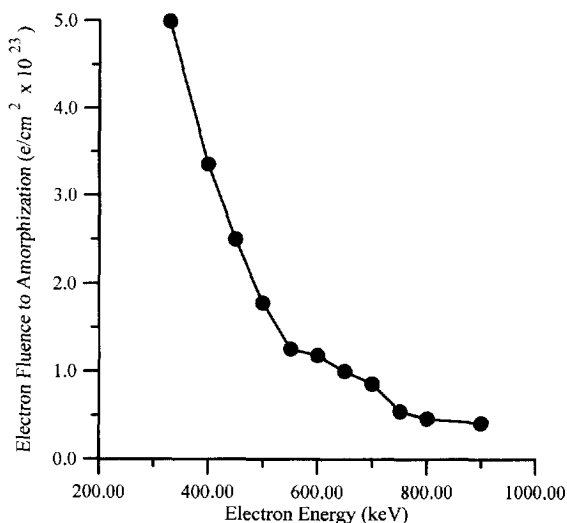
Fig. 12. Energy dependence of the dose-to-amorphization in ZrCr_2 during electron irradiation at 25 K.
