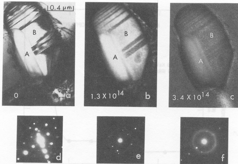
FIGURE 1: Bright-field electron micrographs (a,b,c) and corresponding diffraction patterns (d,e,f) of Zr(Cr,Fe)_2 (A) and Zr_2(Ni,Fe) (B) precipitates in Zircaloy-4 irradiated at 500 K with 350 keV ^{40}Ar ions. Irradiation doses were 0 (a,d), 1.3 \times 10^{14} ions cm^{-2} (b,e) and 3.4 \times 10^{14} ions cm^{-2} (c,f).
