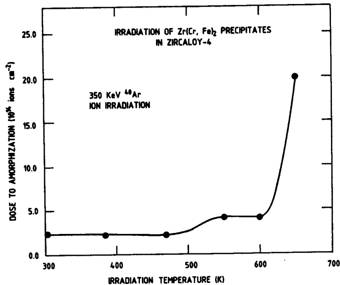
FIGURE 3: Irradiation dose required to produce amorphization versus irradiation temperature for 350 keV ^{40}Ar ion irradiation of Zr(Cr, Fe)_2 precipitates in Zircaloy-4.
