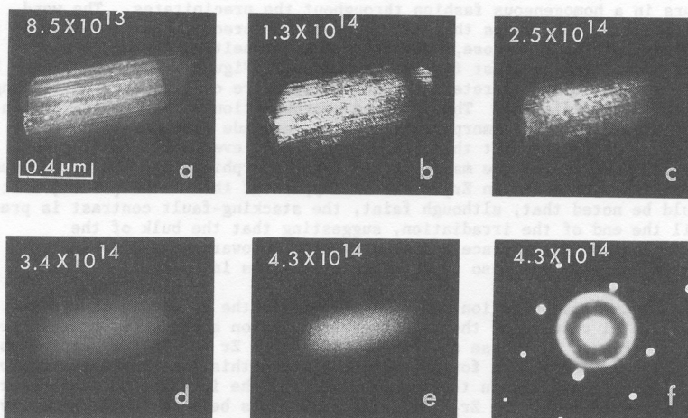
FIGURE 2: Dark-field electron micrographs (a-e) and diffraction pattern (f) of a Zr(Cr,Fe)_2 precipitate in Zircaloy-4 irradiated at 500 K with 350 keV ^{40}Ar ions to doses of 8.5 \times 10^{13} (a), 1.3 \times 10^{14} (b), 2.5 \times 10^{14} (c), 3.4 \times 10^{14} (d) and 4.3 \times 10^{14} ions cm^{-2} (e,f).
